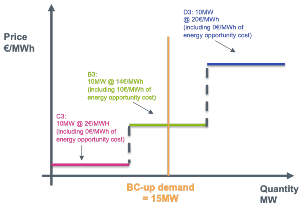
Figure 36: The balancing capacity merit order curve considering bid linking is constructed based on the assumption that the energy part of the co-optimization market results are known, providing insight into the overall market outcomes for balancing capacity.
