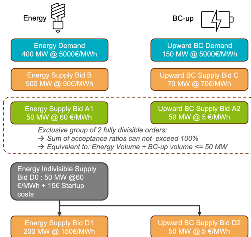
Figure 41: Example with balancing capacity demand causing extramarginal energy bids to be accepted
