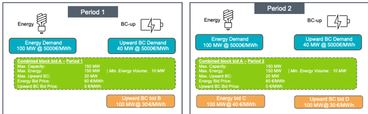
Figure 40: Example with a two-period combined block bid
