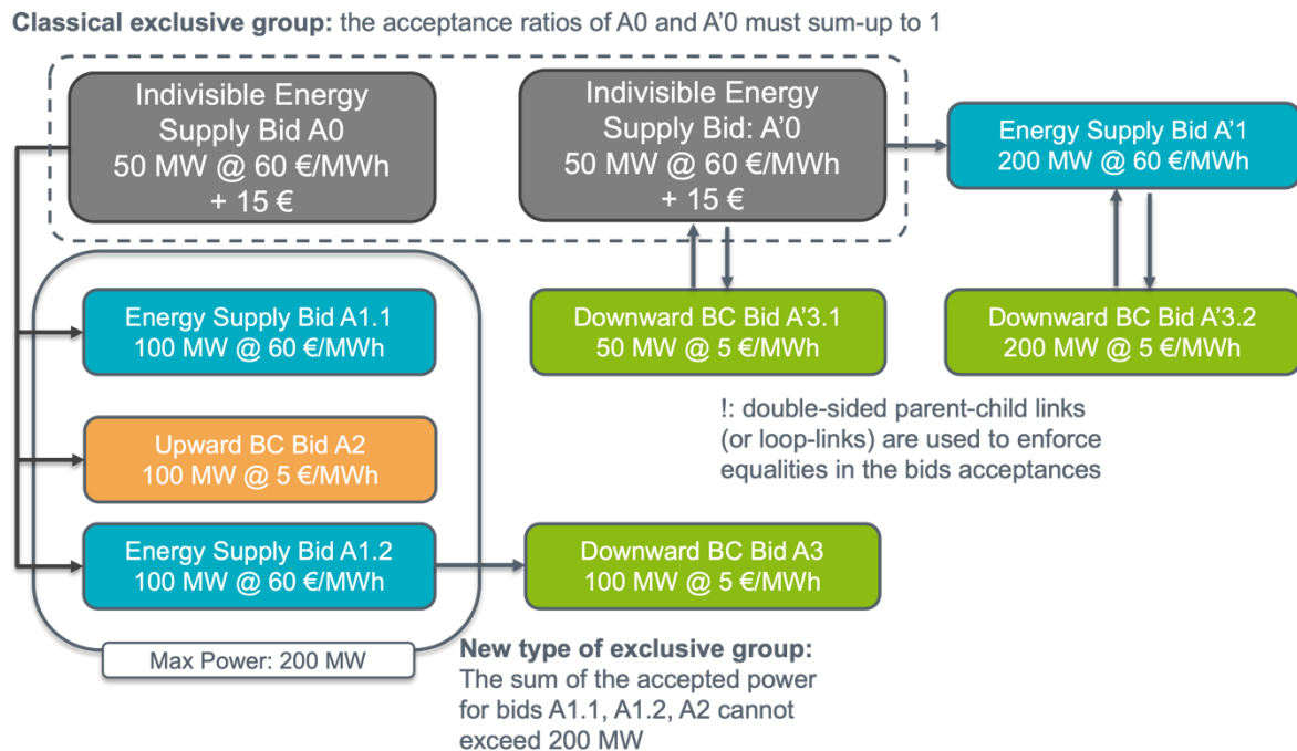
Figure 32: Illustration of a market participant strategy via the unique usage of simple bids and links.
