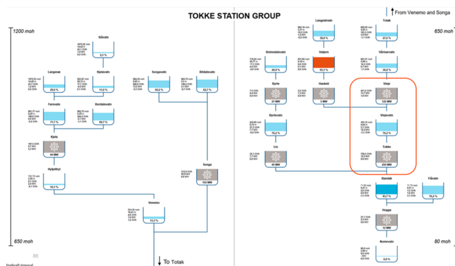
Figure App. C. 2: Hydro system in Southern Norway
