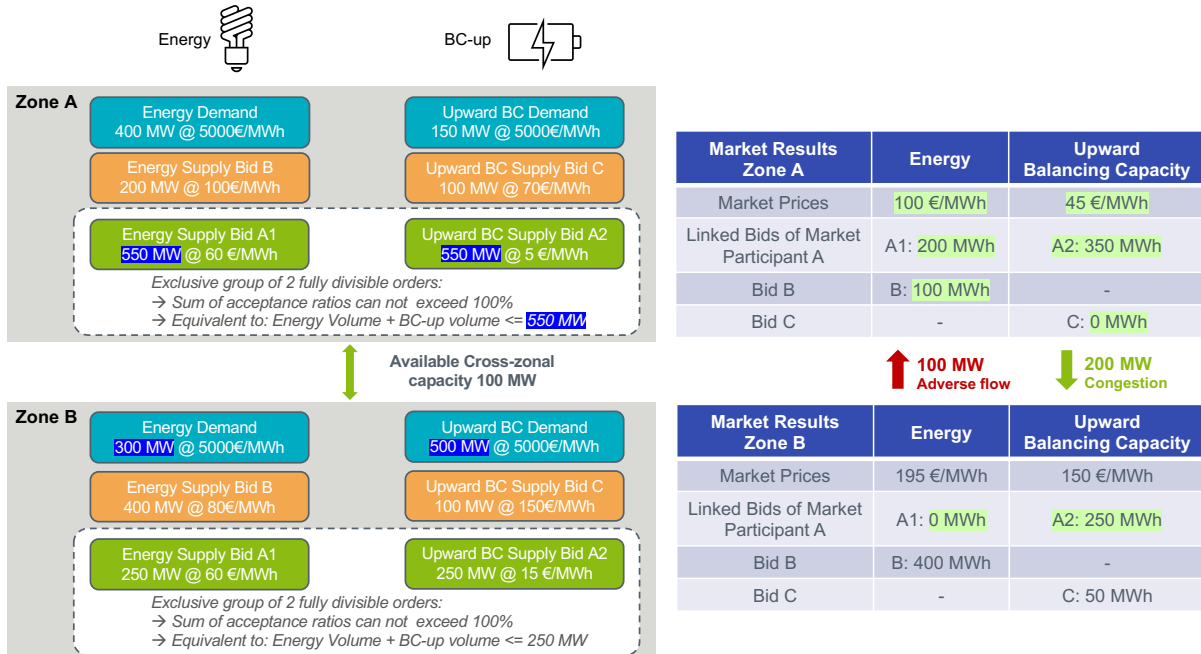
Figure 27: Co-optimized market situation where an adverse energy flow between zones A and B is observed in the optimal solution as it releases further CZC for profitable balancing capacity flows.
