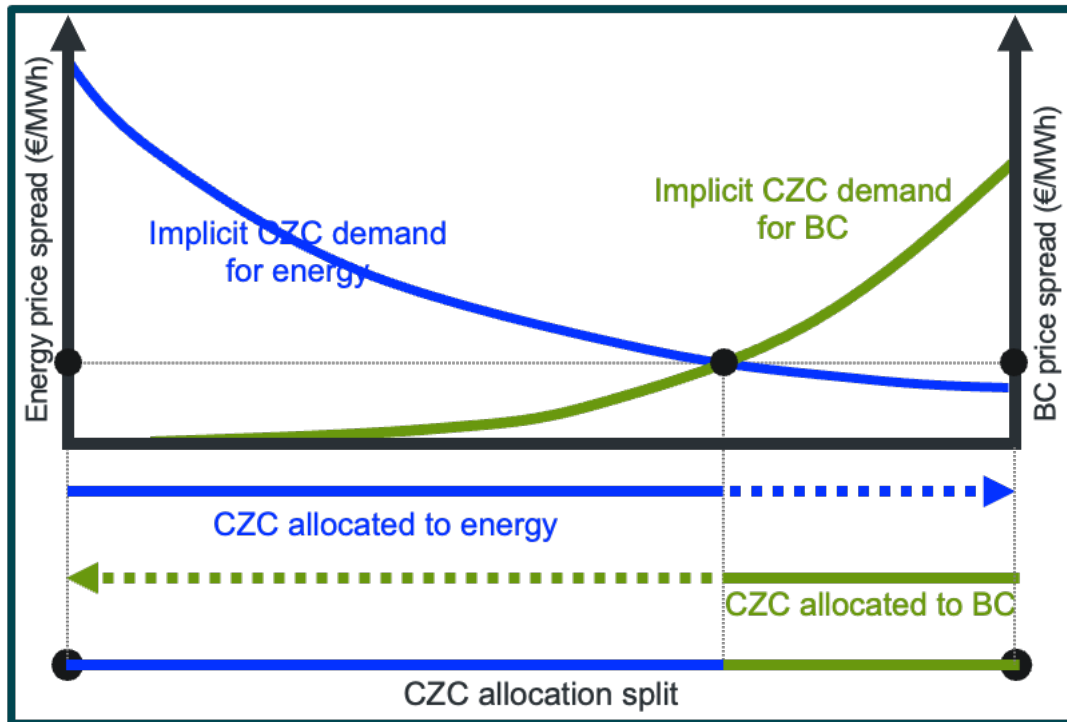
Figure 23: Representation of cross-zonal capacity valuation in a market co-optimizing energy and balancing capacity when the CZC between two zones is allocated to both energy and BC. The blue line represents the implicit CZC demand for energy, and the green line the implicit CZC demand for BC. In this example, the CZC allocation is split between energy and BC. As a result, CZC is valued at the energy and BC price spreads (which must be equal in case of CZC split)
