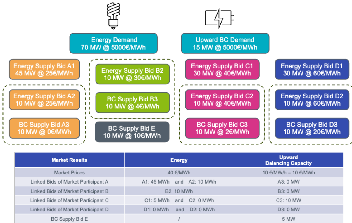
Figure 37: Example presented in Figure 35 enhanced with a balancing-capacity-only bid (bid E).
