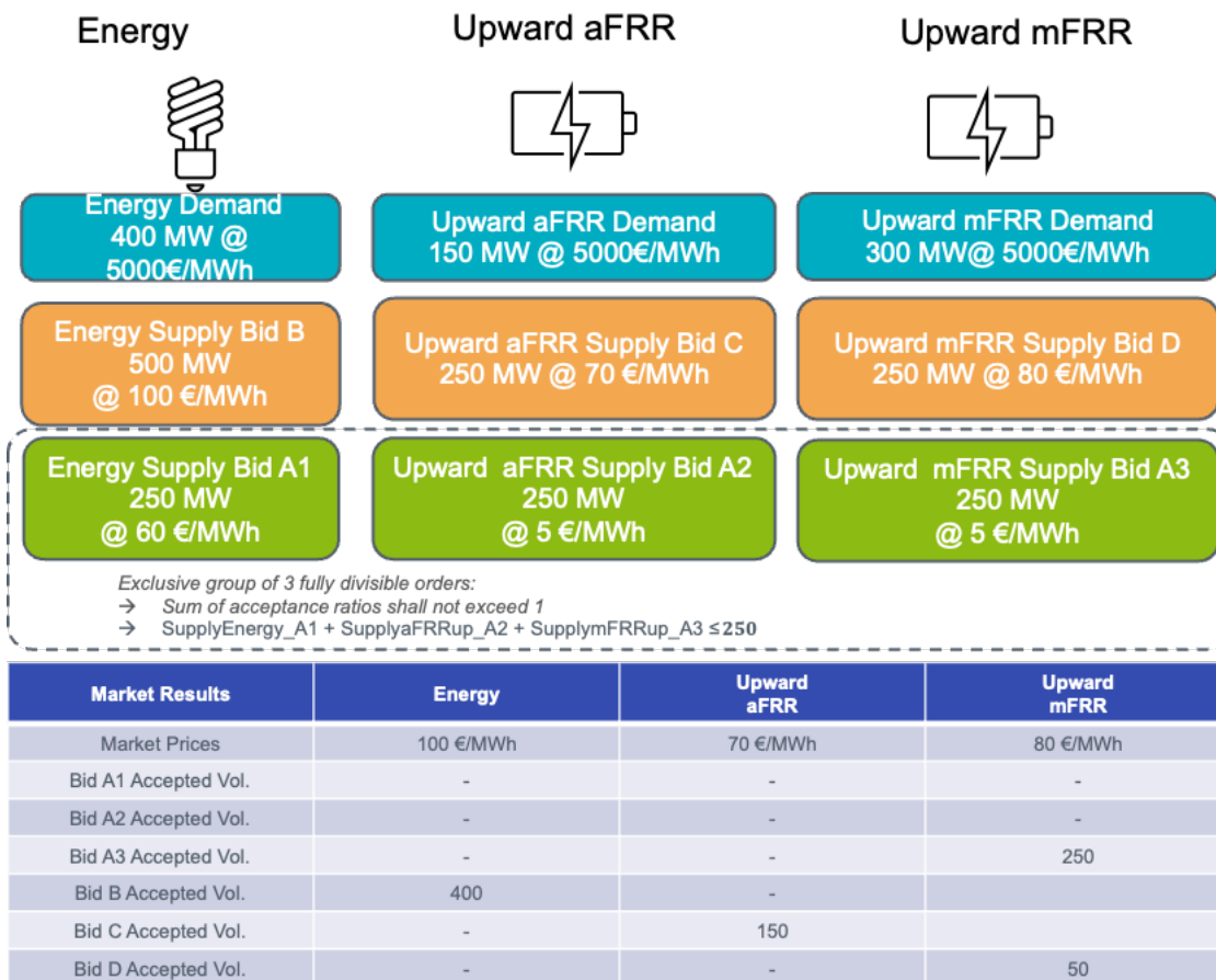
Figure 4: Example 2 - Linked bids for energy and multiple reserve products of the same direction (upward in the Example)
