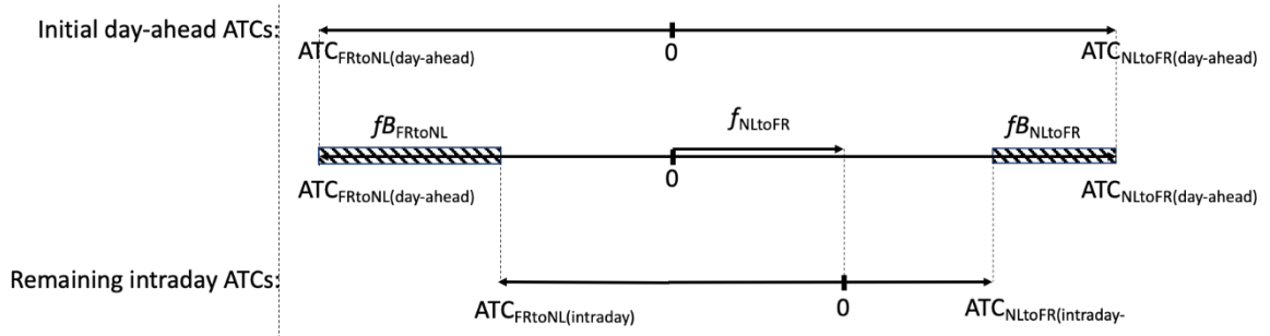
Figure 26: The graphical intuition of the difference between cross-zonal allocation for balancing capacity and energy is that a CZC allocation to balancing capacity (i.e. f_{B_{FRtoNL}} and f_{B_{NLtoFR}} ) implies reserving “positive bandwidths of CZC”,
