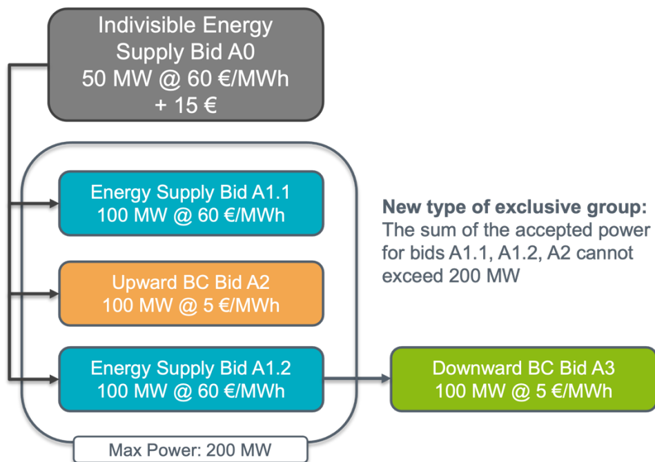
Figure 42: An example of a simple combined bid summarizing several linked bids
