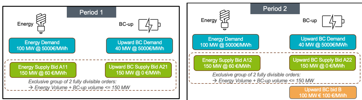
Figure 39: Example illustrating the impact of intertemporal constraints on the acceptance of linked energy and balancing capacity offers and price formation using ramping constraints.
