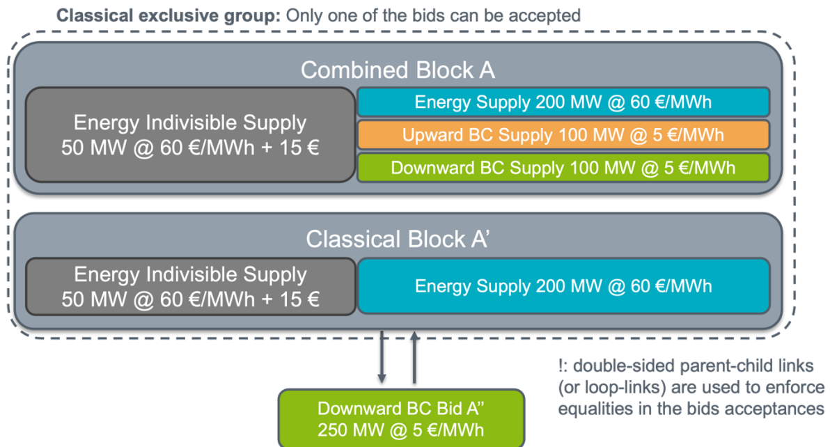
Figure 33: Representation of the bidding strategy of Figure 32 by means of links between combined bids.
