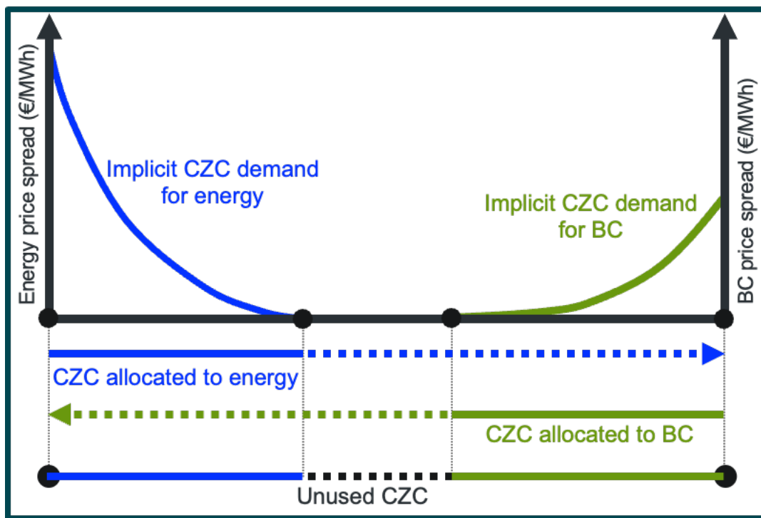
Figure 21: Representation of cross-zonal capacity valuation in a market co-optimizing energy and balancing capacity when the CZC between two zones is not fully utilized. The blue line represents the implicit CZC demand for energy, and the green line the implicit CZC demand for BC. In this example, both demands are fully satisfied by the offered CZC. As a result, the total CZC is not fully used, and the CZC has no value (i.e. no price difference in either energy or BC).
