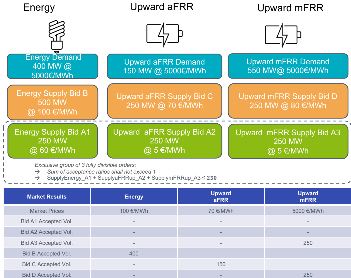
Figure 30: Example without reserve substitutability, where scarcity of mFRR supply results in the mFRR price reaching the price cap set by the price of inelastic demand
