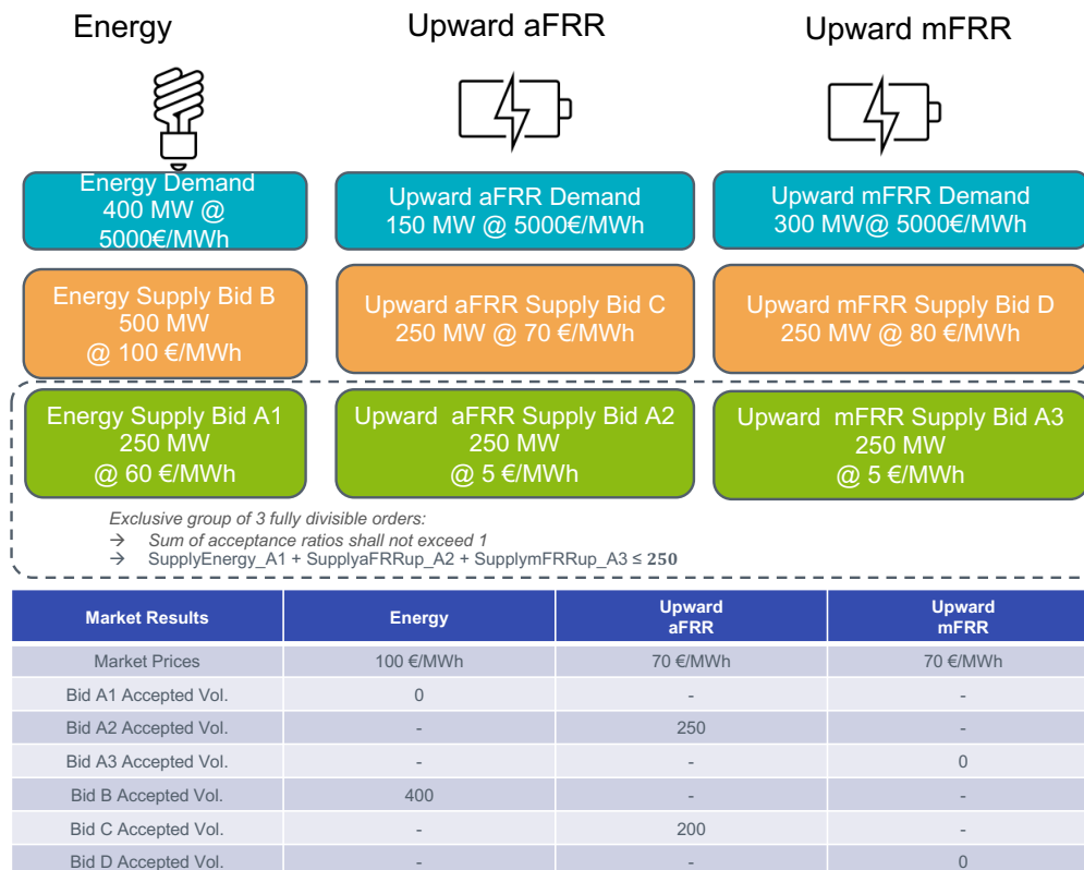
Figure 34: Illustration of the substitutability principle for avoiding price reversals.
