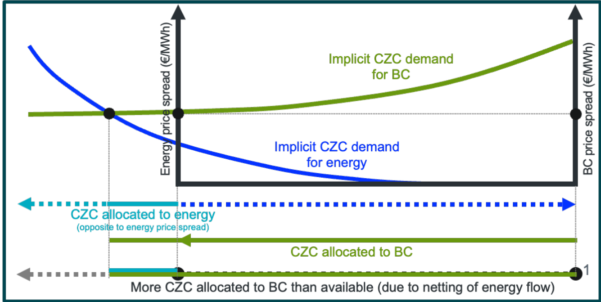
Figure 25: Representation of cross-zonal capacity valuation in a market co-optimizing energy and balancing capacity when the CZC between two zones is fully allocated to BC. The blue line represents the implicit CZC demand for energy, and the green line the implicit CZC demand for BC. In this example, the implicit CZC demand for BC exceeds the CZC demand for energy. As a result, energy flow is allocated against the price difference to enable (through netting) further CZC allocation to the more valuable BC. Cross-zonal capacity is valued at the resulting price spread (which is equal for BC and for energy)
